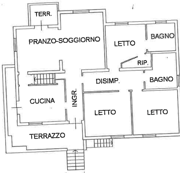
PIANO TERRA H=3,00
